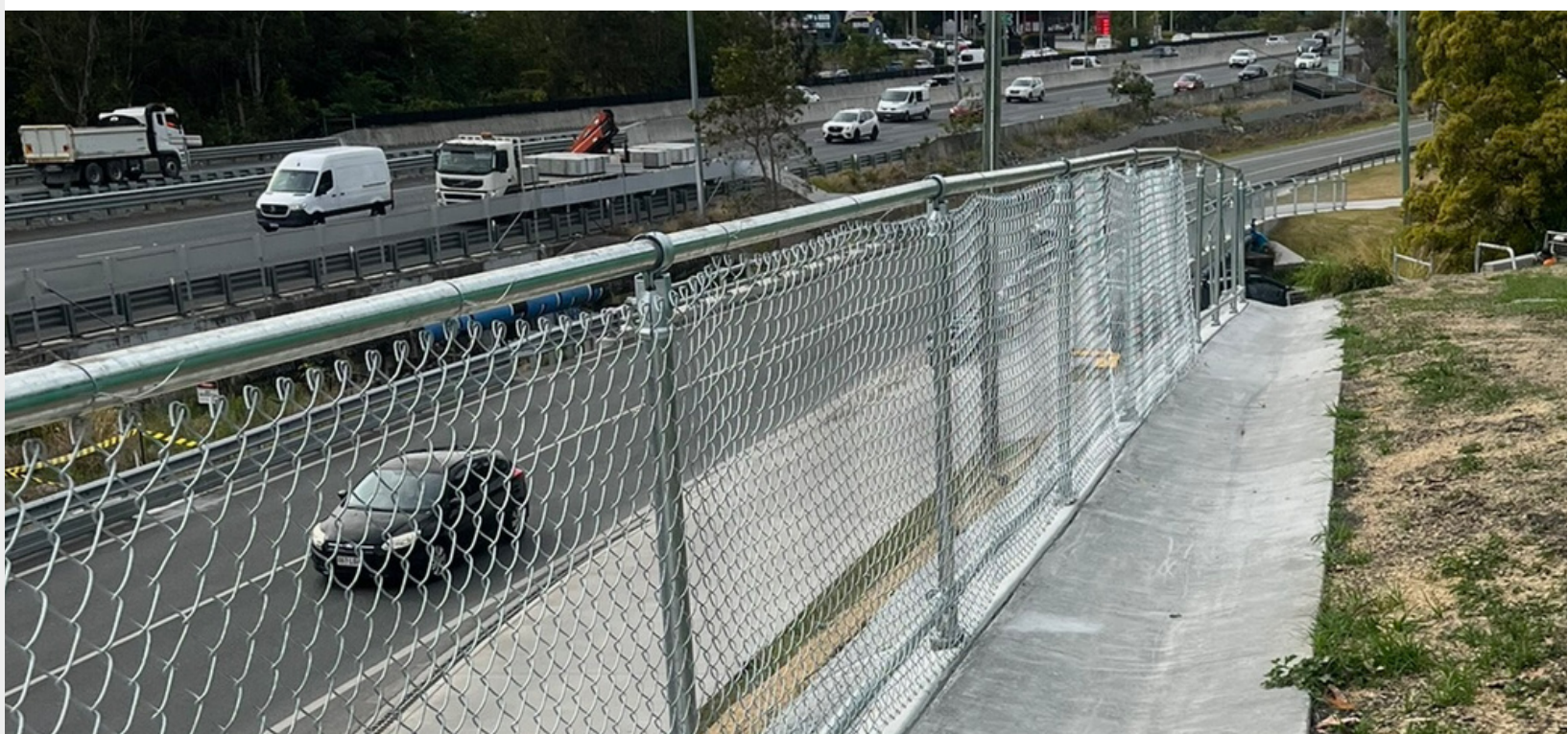
1200mm galvanised chainwire used as fall protection
